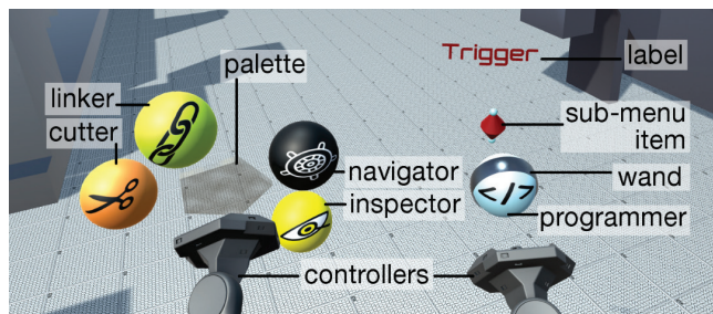
Figure 4: Ivy’s Wand and Palette menu system.
