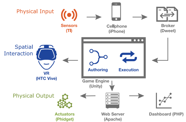
Figure 2: Ivy system overview.
